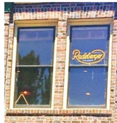
Note tie plates in place as well as the arched spandrel above the upper window. A lintel can be noted above the double windows to provide reinforcement and serve as a small header.
